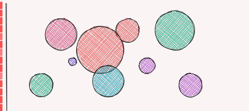
Bubble
