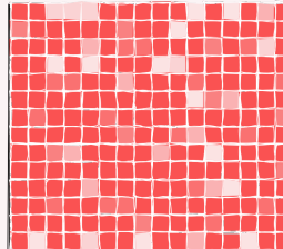
Cartesian heatmap
