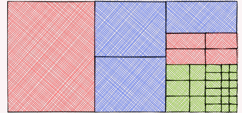
Tree Map
